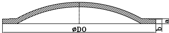
Blank Flange form (DN350 up to DN2600)
